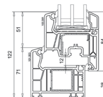
INEO 76 (AD)
